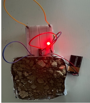
Soil moisture sensor testing clay soil
